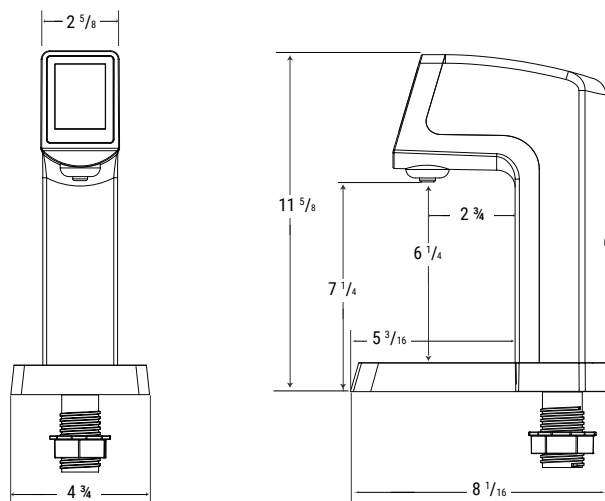
Above Counter with Drip Tray
