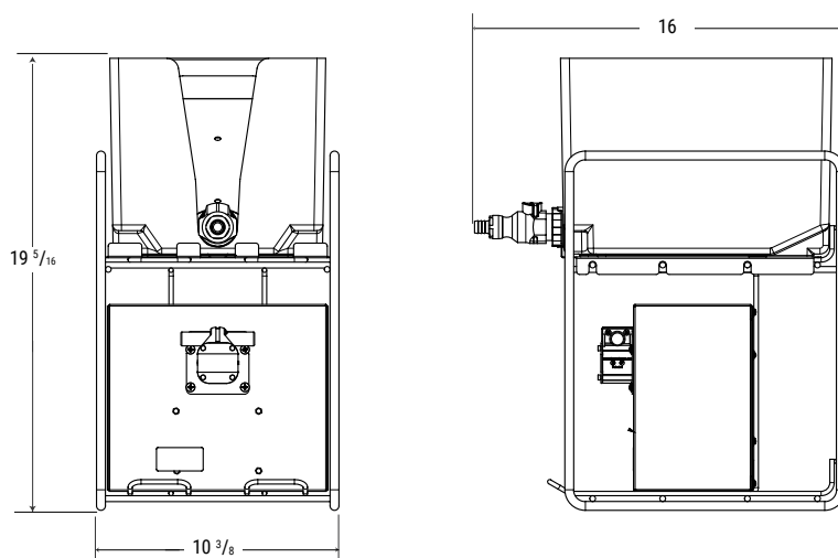
Below Counter - Pouch Model
