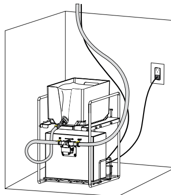
Single+ Below Counter Pouch Model
